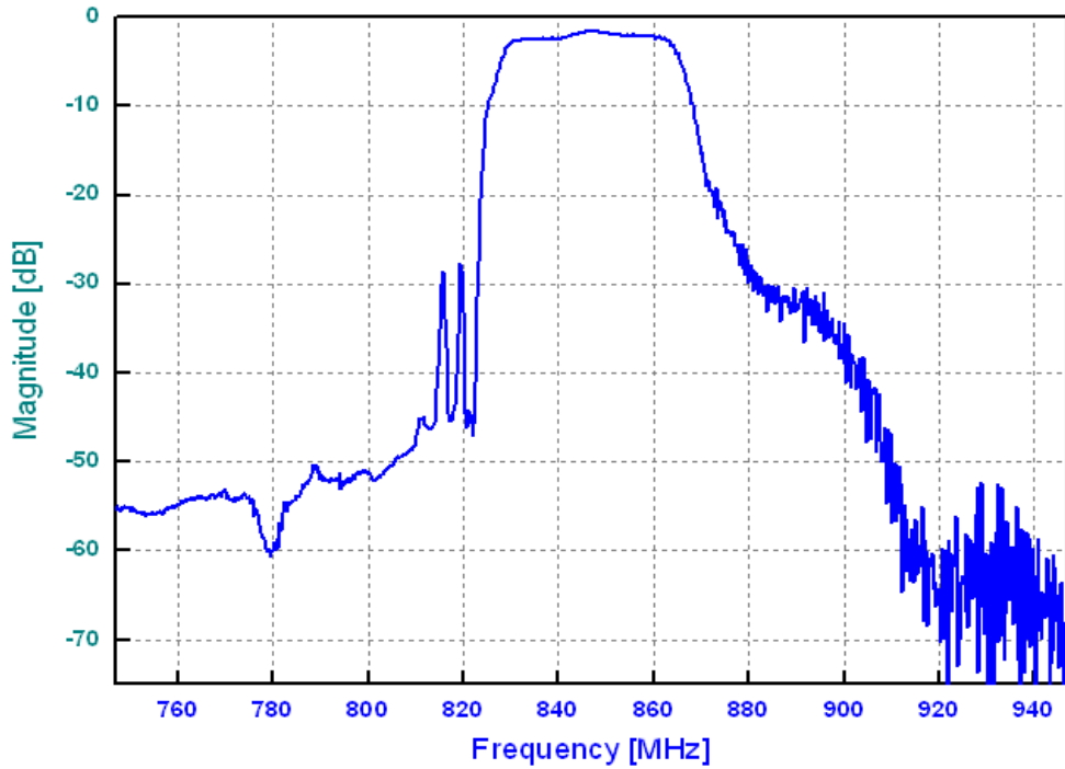
Frequency Response
